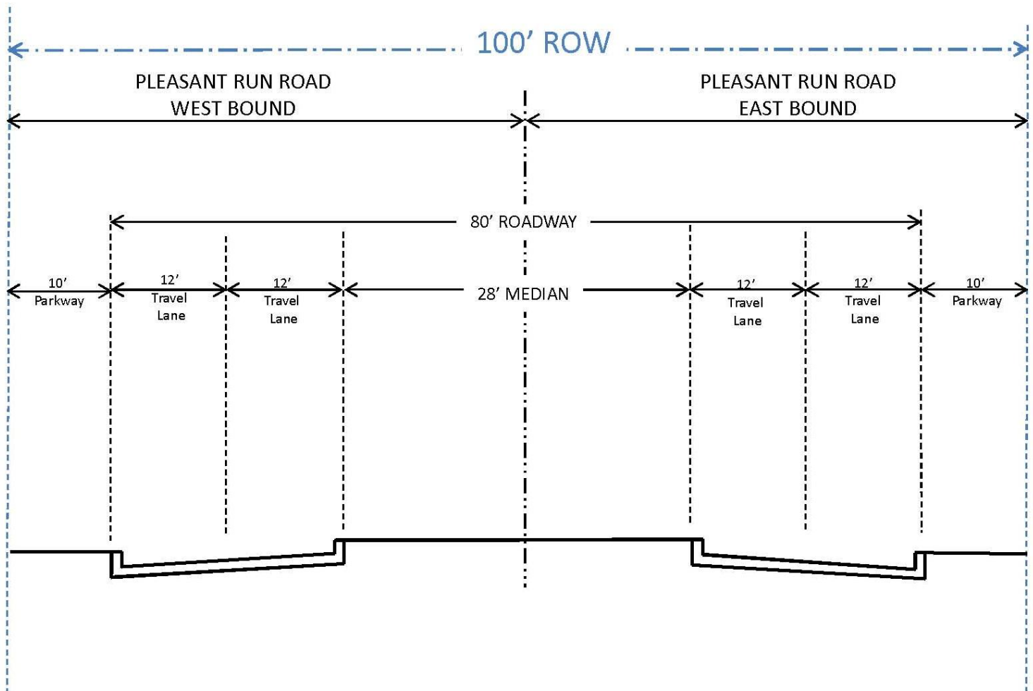
Figure 1: City of Lancaster Master Thoroughfare Plan 2006 Major Arterial Type B
