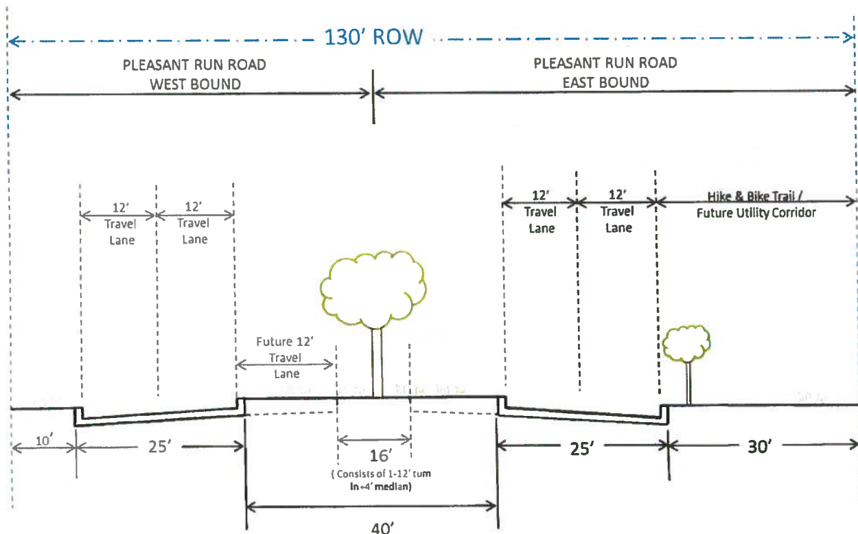
Figure 5: Pleasant Run Road (from Lancaster-Hutchins Road to Millers Ferry Road)
