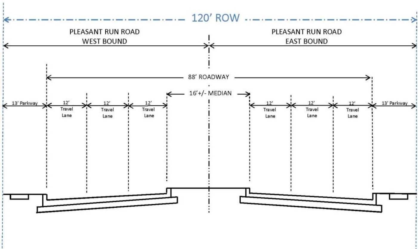
Figure 3: Existing Pleasant Run Road (West of Lancaster-Hutchins Road)
