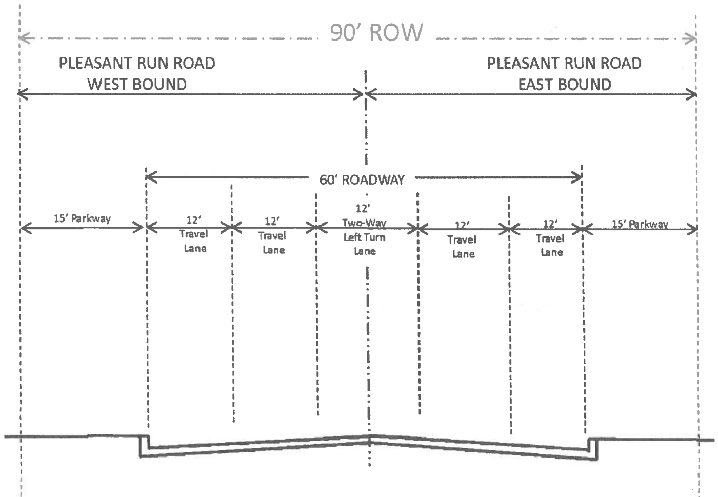
Figure 2: City of Wilmer Master Community Plan 2030 Minor Thoroughfare 'B'
